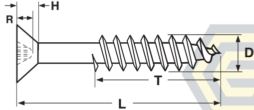
FLAT PHILLIPS DEEP THREAD WOOD SCREW
