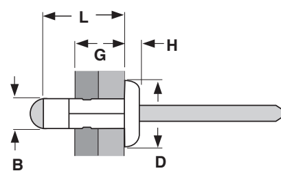
DOME HEAD
