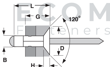
COUNTERSUNK
