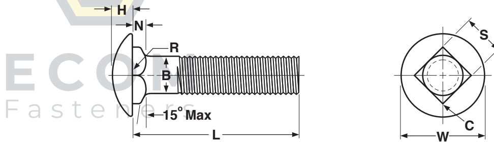
CARRIAGE BOLTS, SHORT NECK
